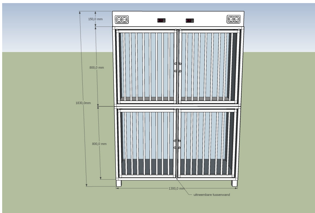
A4: 2x BOX L 1300x800x720MM WITH REMOVABLE WALL, FLOORHEATING, ON WHEELS
